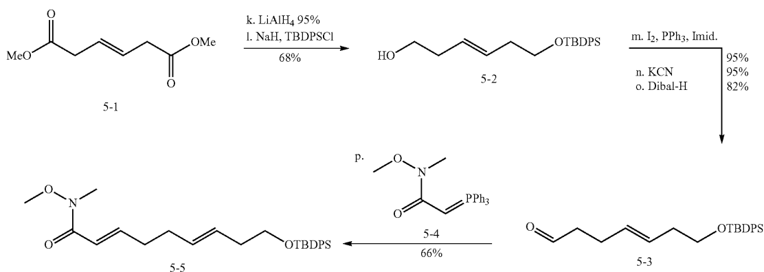
Scheme 5: Preparation of Weinreb amides
