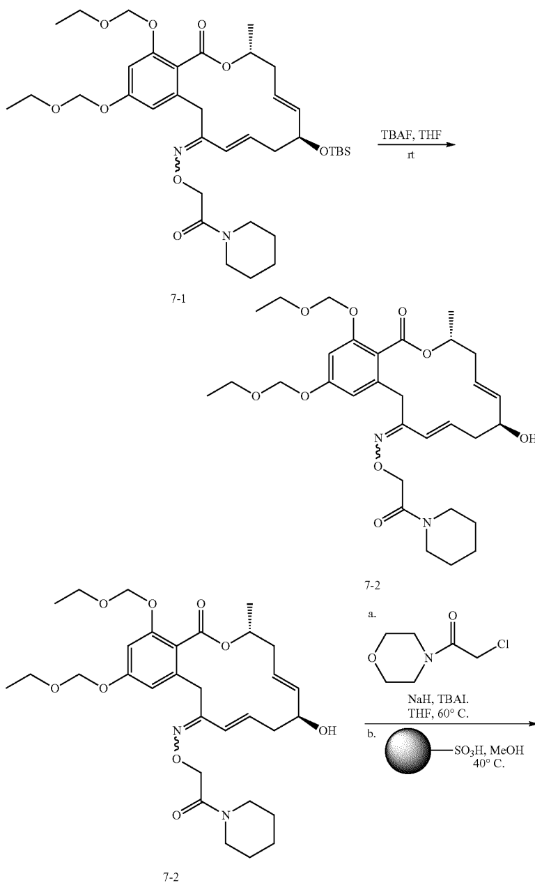
Scheme 7: Derivatives of hydroxy-substituted macrocycles
