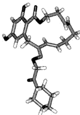
Wire-frame representation of crystal structure of compound 13b
