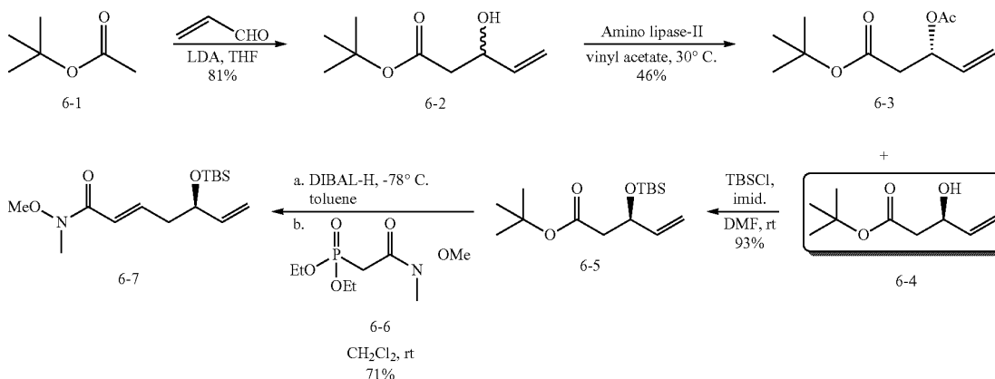
Scheme 6: Synthesis of hydroxy-substituted Weinreb amides
