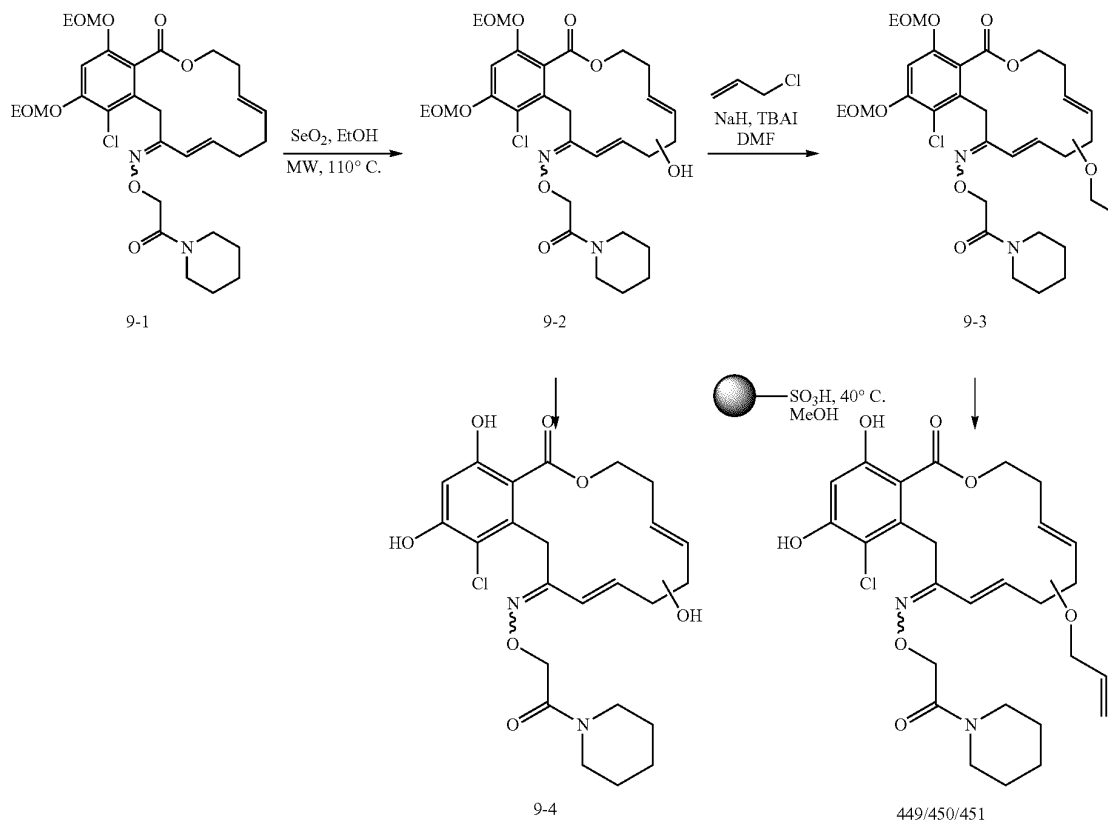
Scheme 9: Allylic oxidation of macrocycles
