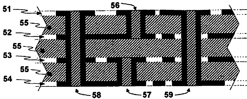
Figure 5. Composition of the PCB for the Capacitive Touch Pad Sensor
