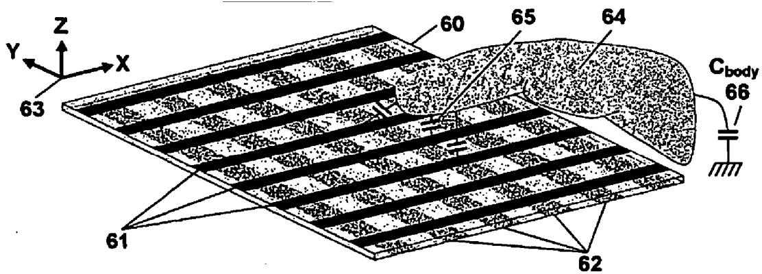
Figure 6. Conceptual Capacitive Touch Pad Sensor
