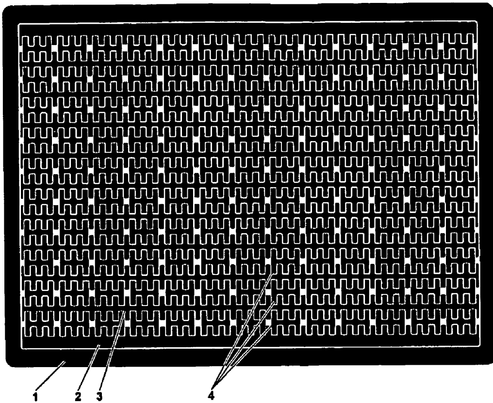
Figure 1. Artwork for the First (Top) Copper Layer
