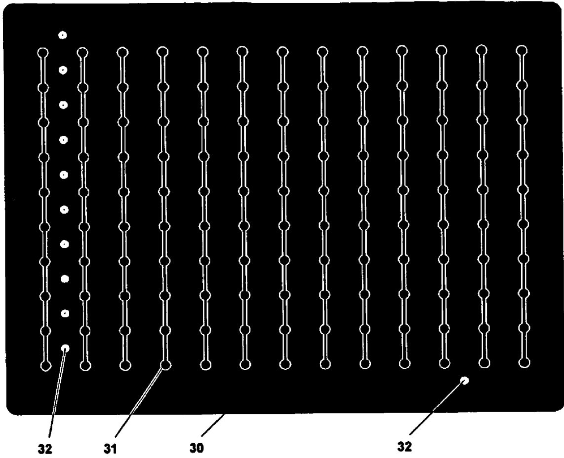
Figure 3. Artwork for the Second (Internal) Copper Layer
