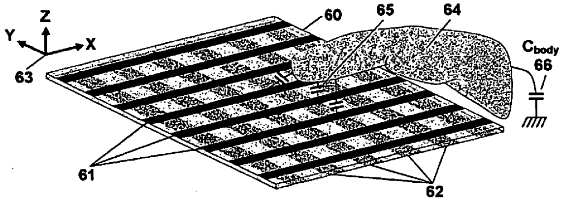
Conceptual Capacitive Touch Pad Sensor
