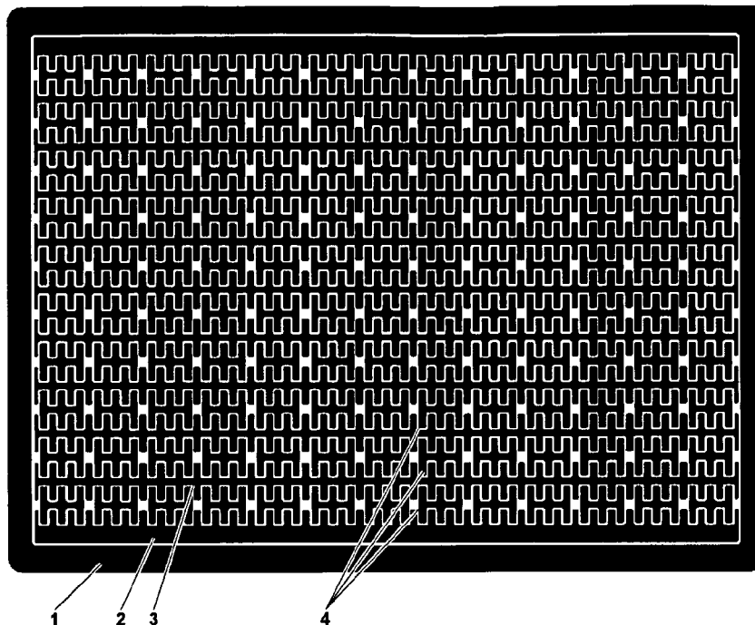
Artwork for the First (Top) Copper Layer
